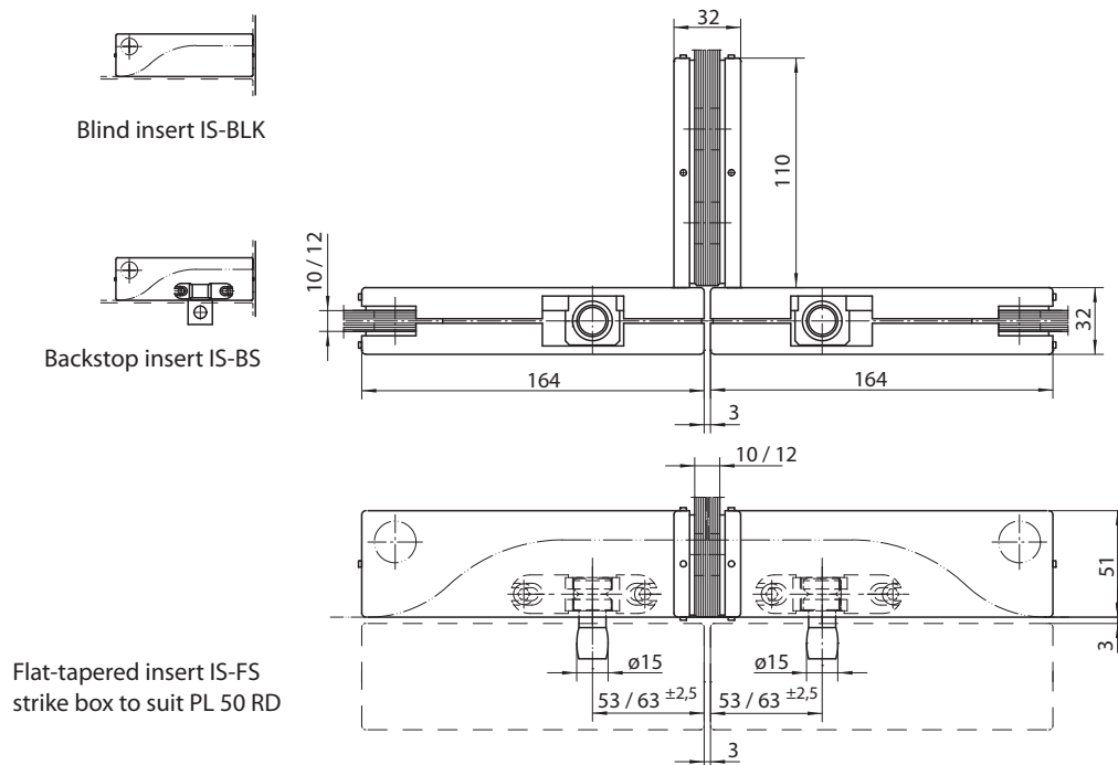
Drawing no. 91905-1-0108
