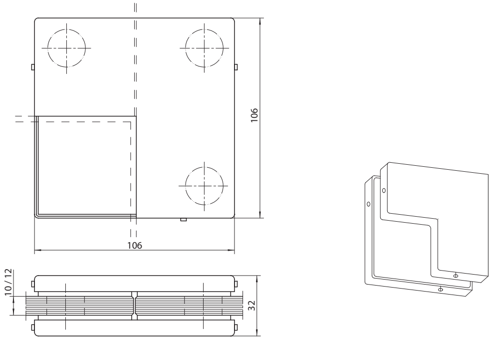
Drawing no. 91905-1-0109
